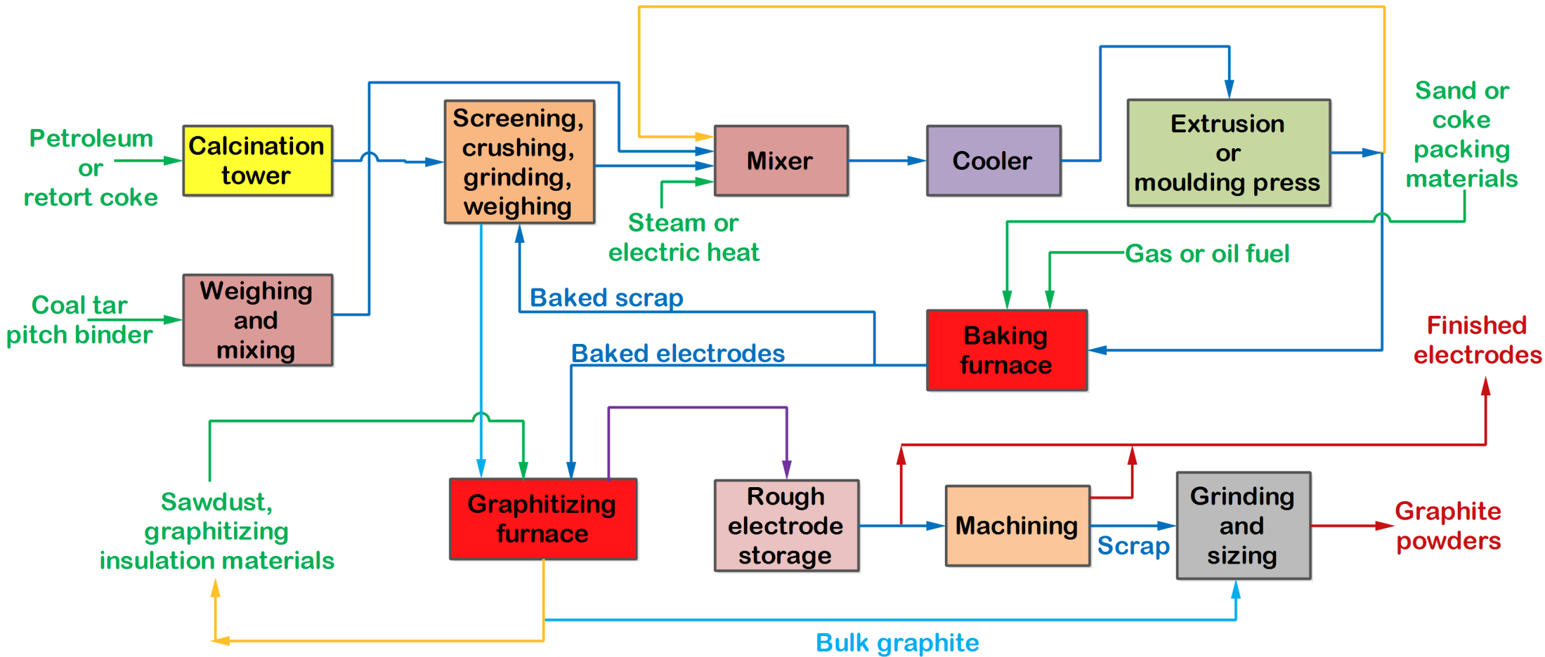
Figure: Manufacture of Graphite from retort or petroleum coke
